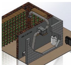
Wall Mount
