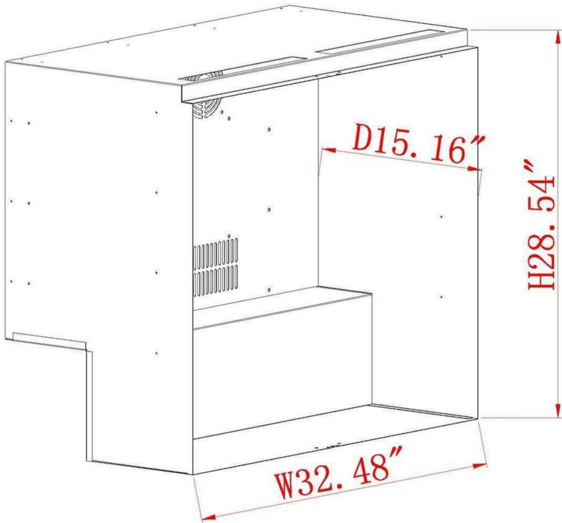
Interior Cabinet Dimensions in inches
