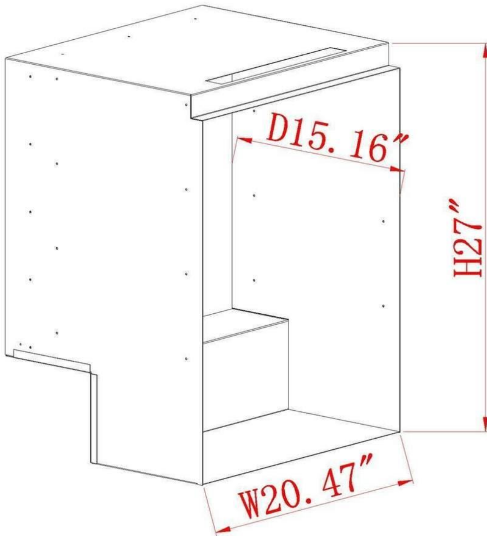
Interior Cabinet Dimensions in inches
