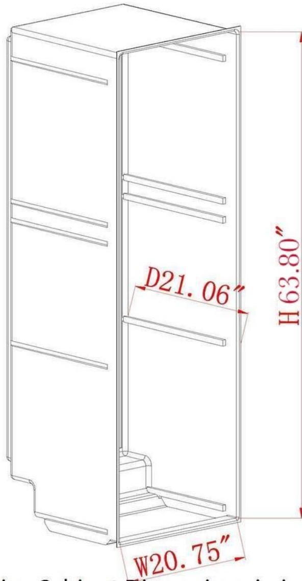
Interior Cabinet Dimensions in inches
